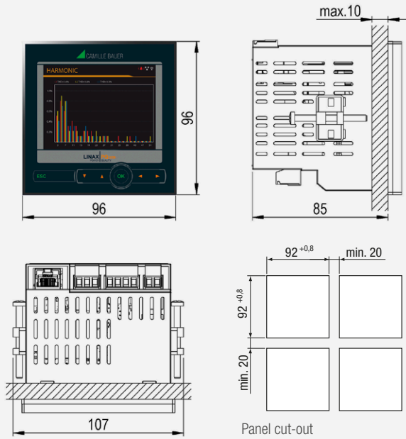
DIMENSIONAL DRAWING PQ1000-1
