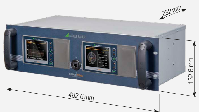
DIMENSIONAL DRAWING PQ5000-RACK
