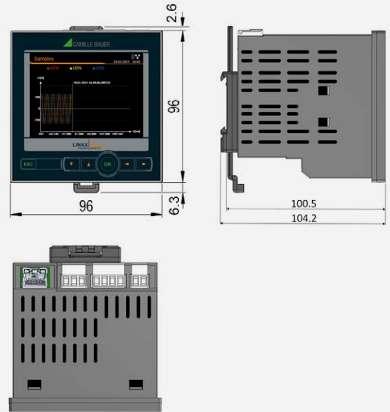
DIMENSIONAL DRAWING PQ1000-2
