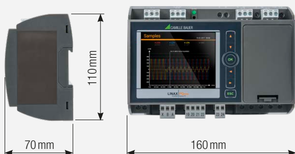
DIMENSIONAL DRAWING PQ5000
