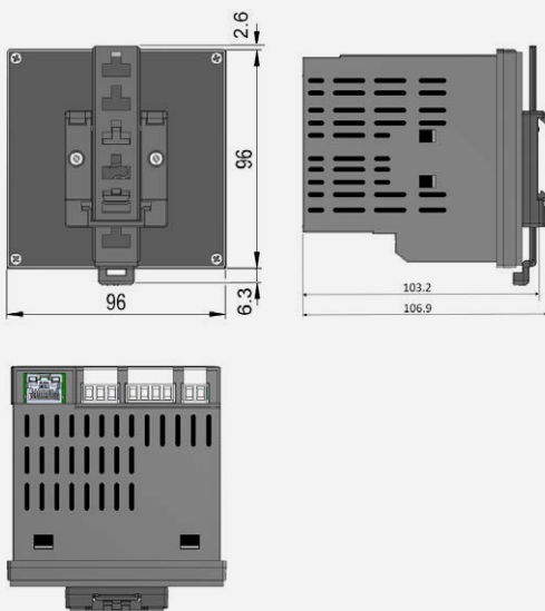
DIMENSIONAL DRAWING PQ1000-3
