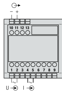
Fig. 3. Power supply internal from measuring input, power supply not required.
