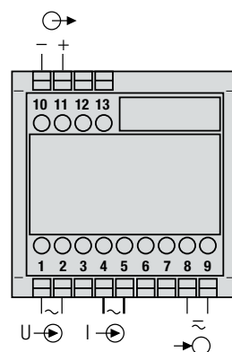
Fig. 2. Power supply to terminals 8 and 9.
