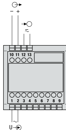
Fig. 4. Power supply connected to the low tension terminal side 12 and 13.
