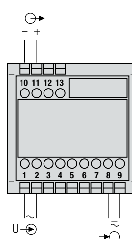
Fig. 2. Power supply connected to terminals 8 and 9.
