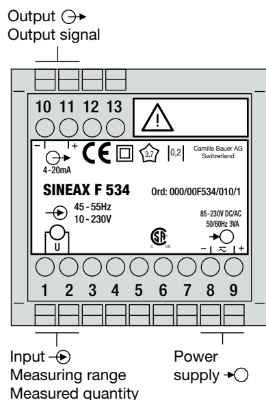
Fig. 5. Declaration to type label.
