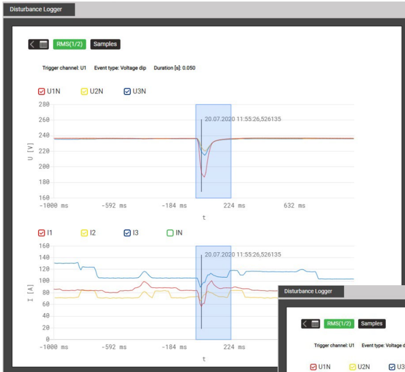
Graphical display of a disturbance recording
