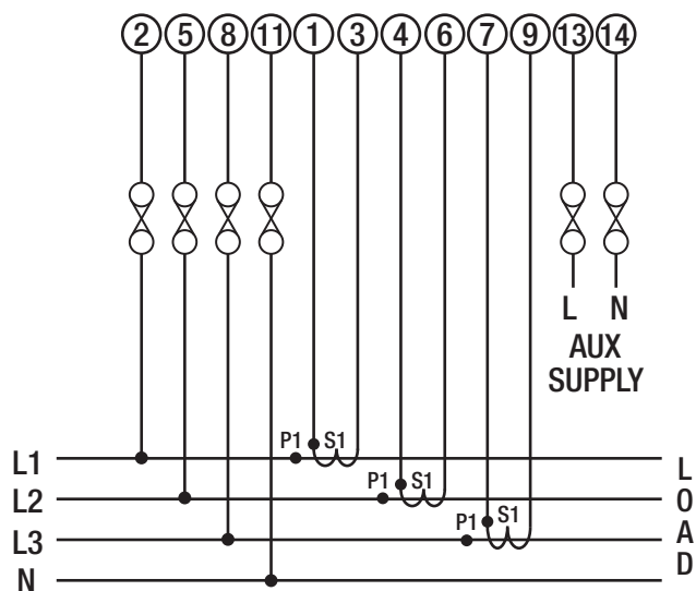
3-Phase 4-Wire unbalanced
