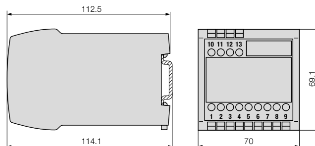
Fig. 8. Housing type P13/70 clipped onto a top-hat rail (35×15 mm or 35×7.5 mm, acc. to EN 50 022).
